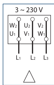
4 Correct connection
