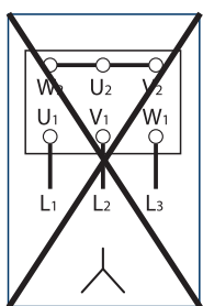
3 Incorrect connection
